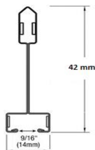
TEE LIDER GROOVE RANURADA ULTRADELGADA 9/16"
